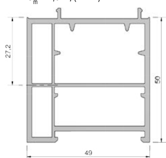
TSUK5049-Steg
